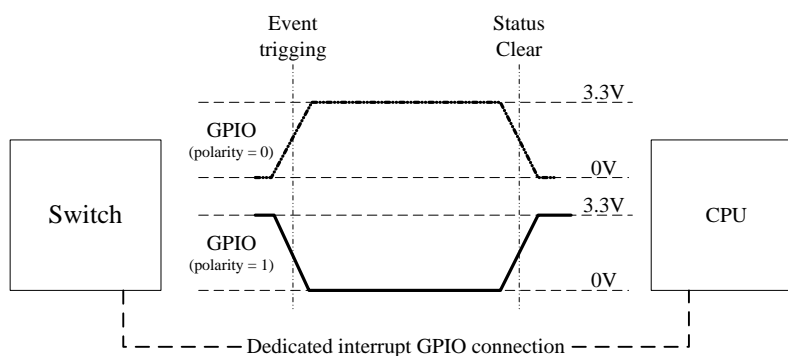
Figure 6. Interrupt Polarity
